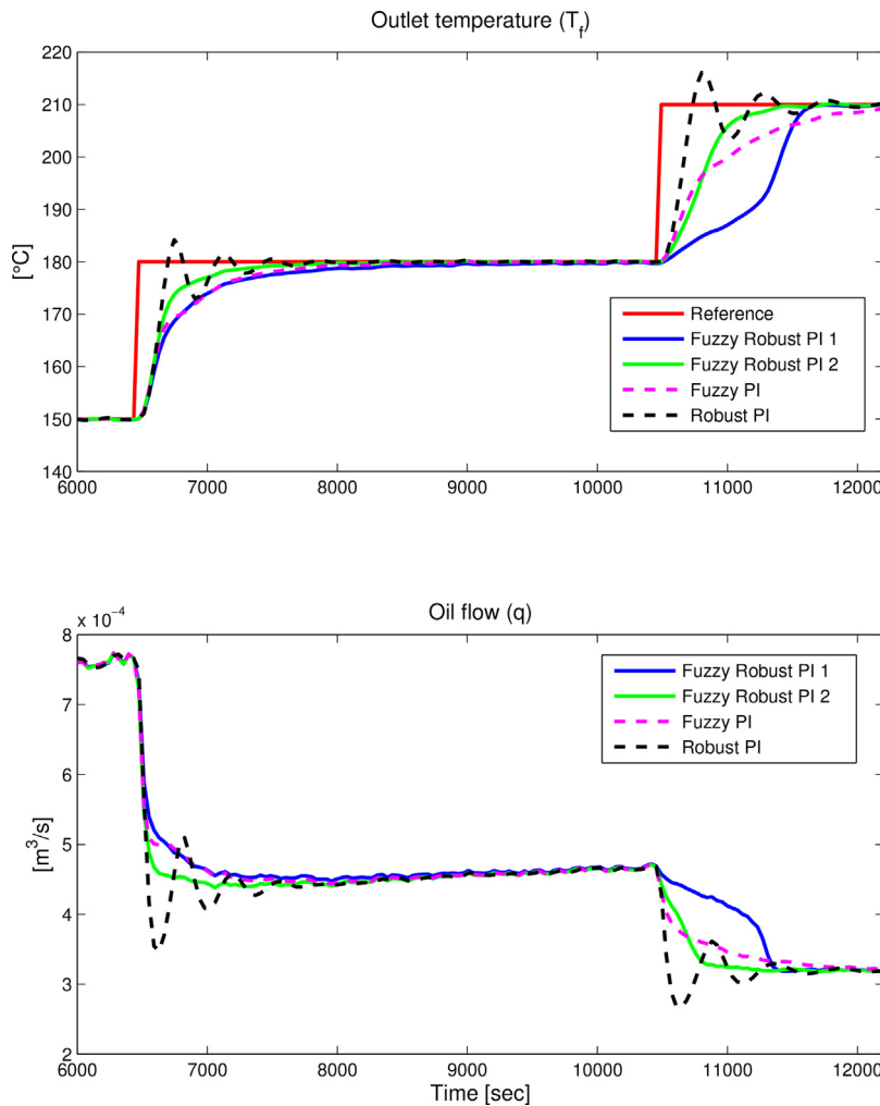
Fig. 6. Results for the controllers under a sunny day.
